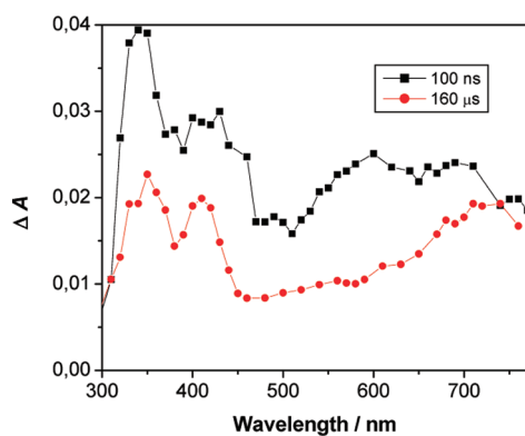
Figure 3. Transient absorption spectra of 9 in \text{O}_2 -purged TFE.
