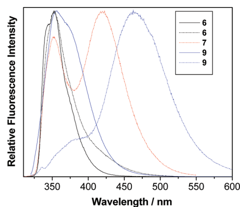
Figure 1. Normalized fluorescence spectra of naphthols 6, 7, and 9 in CH 3 CN (solid line) and CH 3 CN–H 2 O (1:4) (dashed line).
